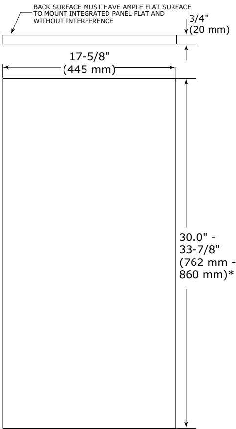
Integrated Panel
