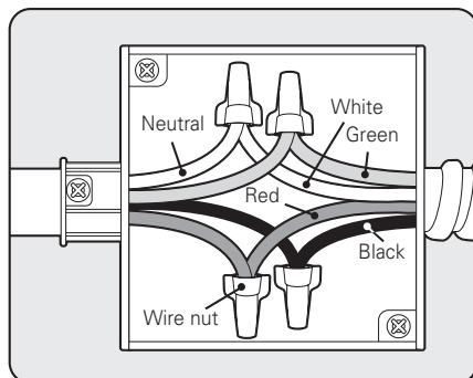
Junction Box
